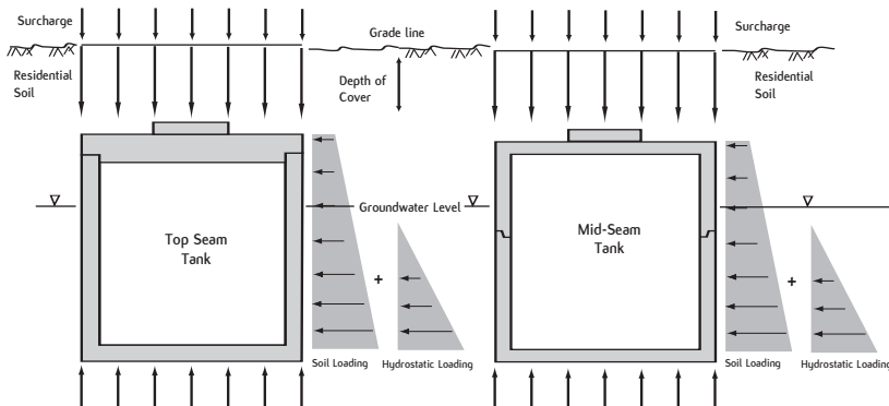
Optional Loading Where Appropriate
