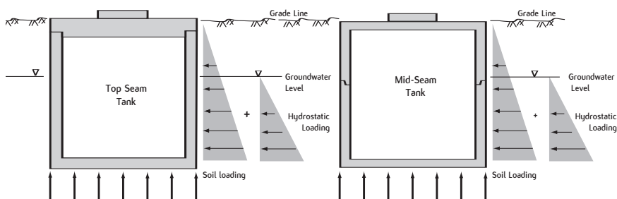
External Soil and Water Loading: Tank Empty
